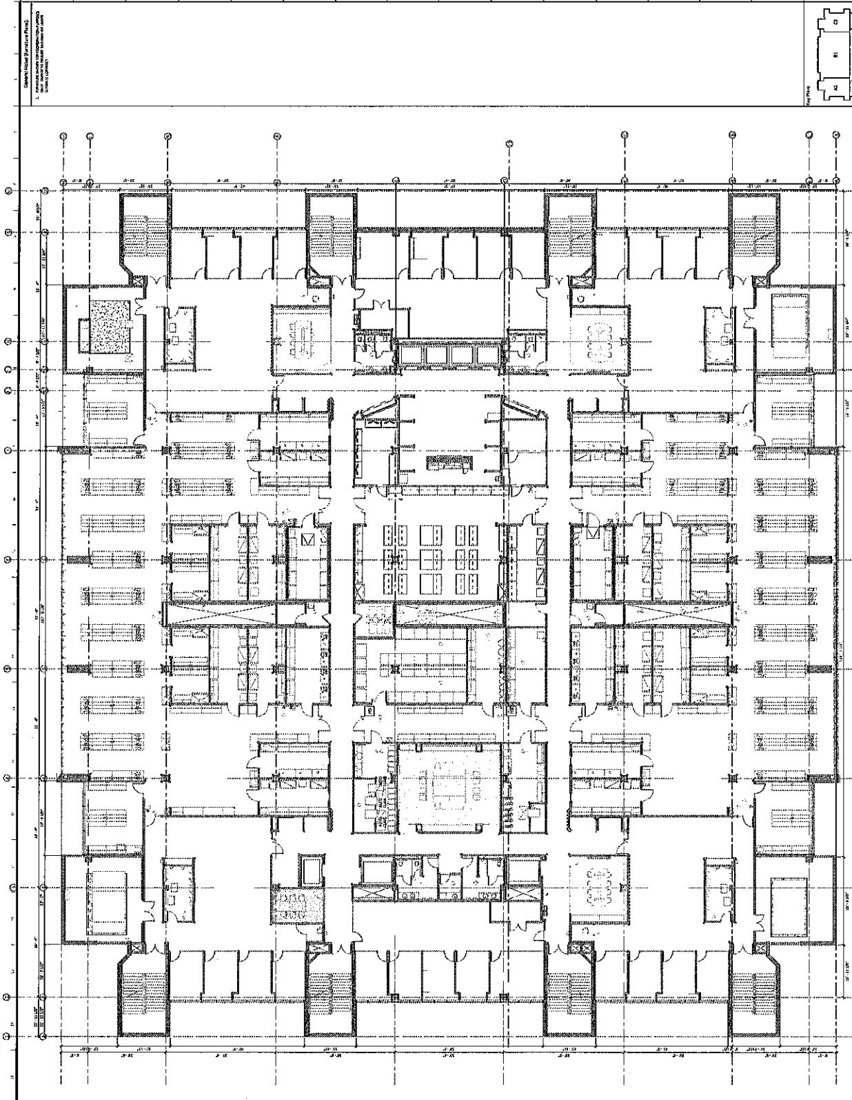
LEVEL 6 - FURNITURE PLAN
