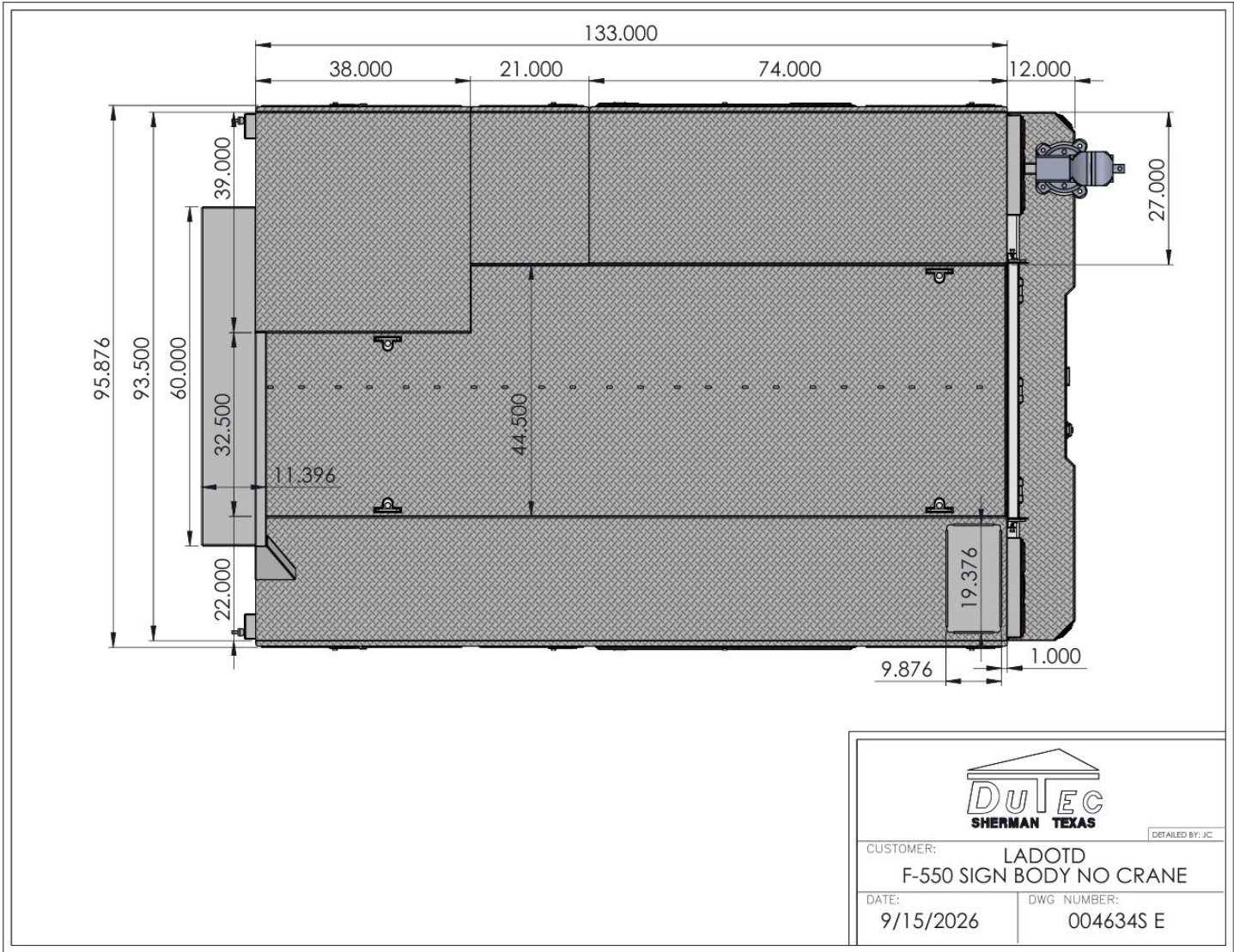
Figure 7 Overhead drawing of utility bed with measurements and dimensions in accordance with specs.
