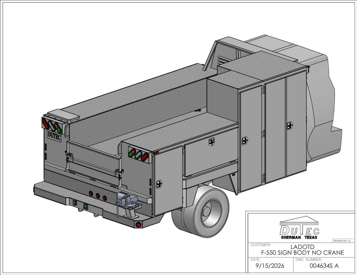
Figure 3 General assembly drawing of utility truck bed.
