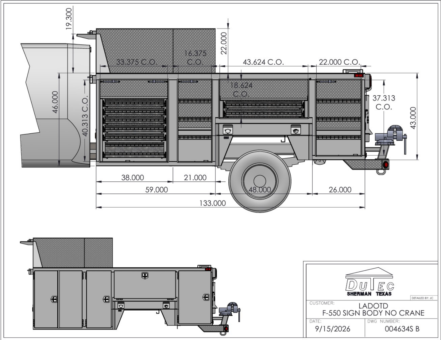
Figure 4 General assembly driver side view drawing with measurements in accordance with specs.
