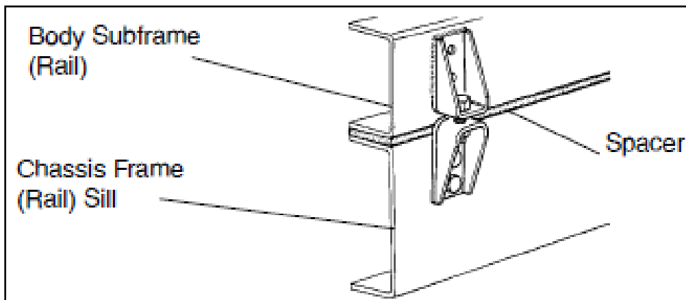
Figure 1 Brackets connecting body with chassis and spacer in between.
