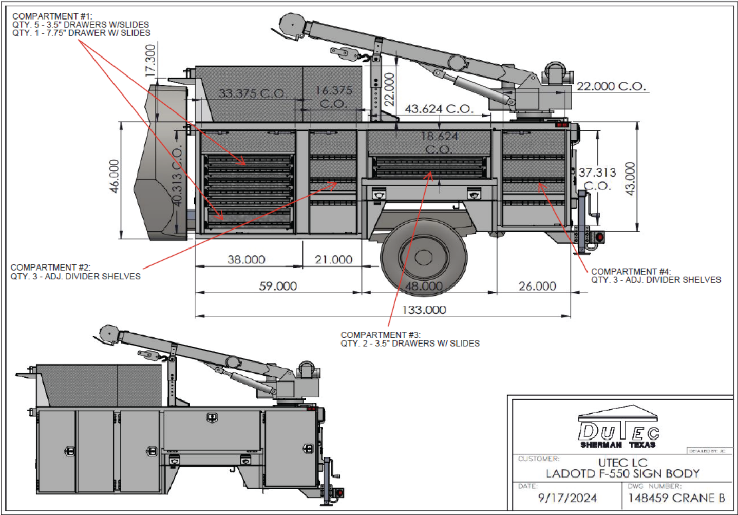
Figure 4 General assembly driver side view drawing with measurements in accordance with specs.
