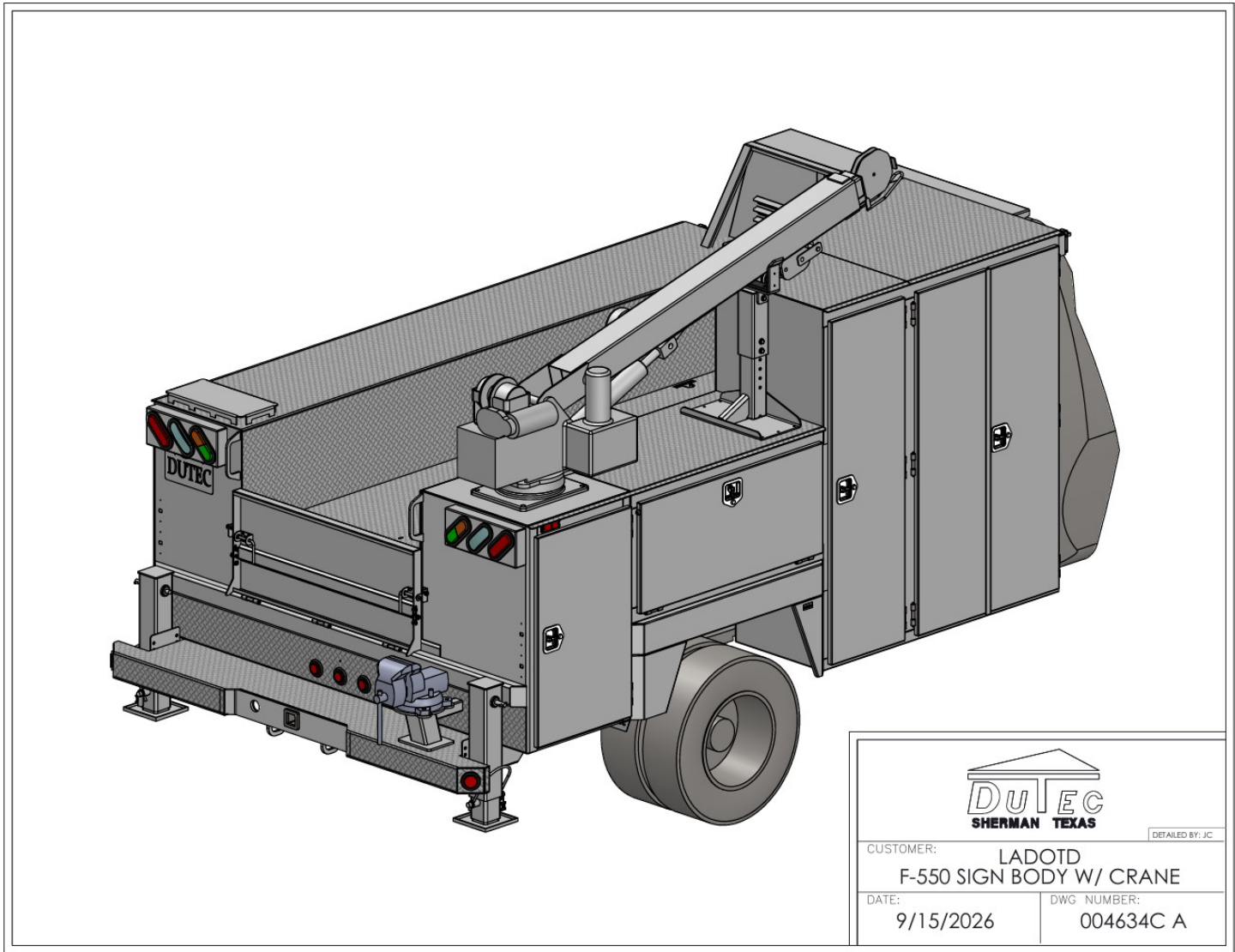
Figure 3 General assembly drawing of utility truck bed with crane.
