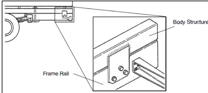
Figure 2 Example of how to attach fishplate.
