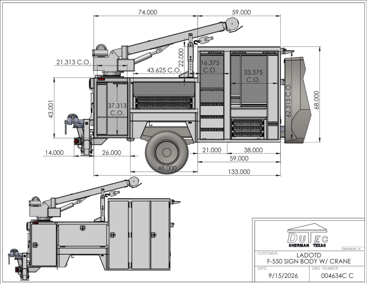
Figure 5 General assembly passenger side view drawing with measurements in accordance with specs.
