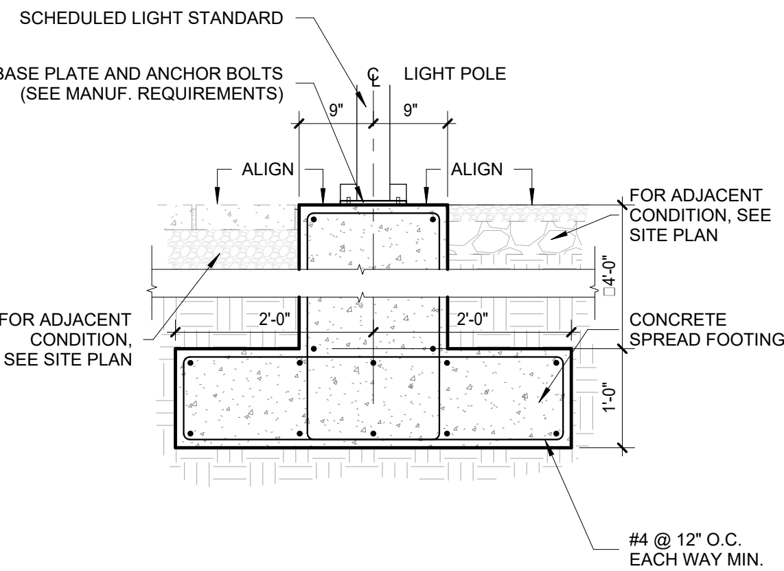
20 LIGHT POLE FOUNDATION 3/4" = 1'-0"
