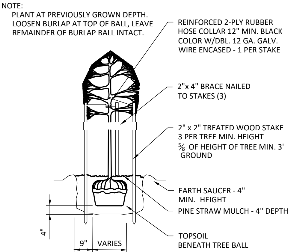
2 TREE STAKING DETAIL N.T.S. (CLASS 'B' TREE)
