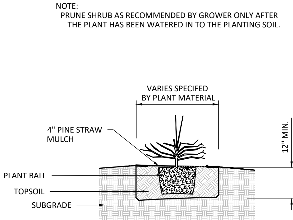
3 CONTAINER SHRUB PLANTING DETAIL N.T.S.
