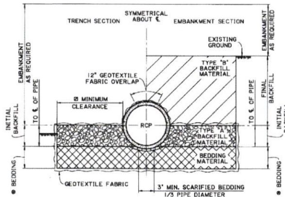
REINFORCED CONCRETE PIPE STORM DRAIN TRENCH AND EMBANKMENT INSTALLATIONS SCALE: 1\frac{1}{2}" = 1'-0"
