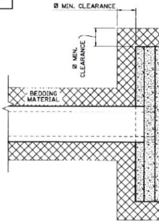
TYPICAL CROSS DRAIN INSTALLATION WITH AND WITHOUT HEADWALL (EMBANKMENT MATERIAL NOT SHOWN FOR CLARITY) NTS
