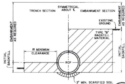
▲ REINFORCED CONCRETE PIPE SIDE DRAIN TRENCH AND EMBANKMENT INSTALLATIONS SCALE: 1\frac{1}{2}" = 1'-0"
