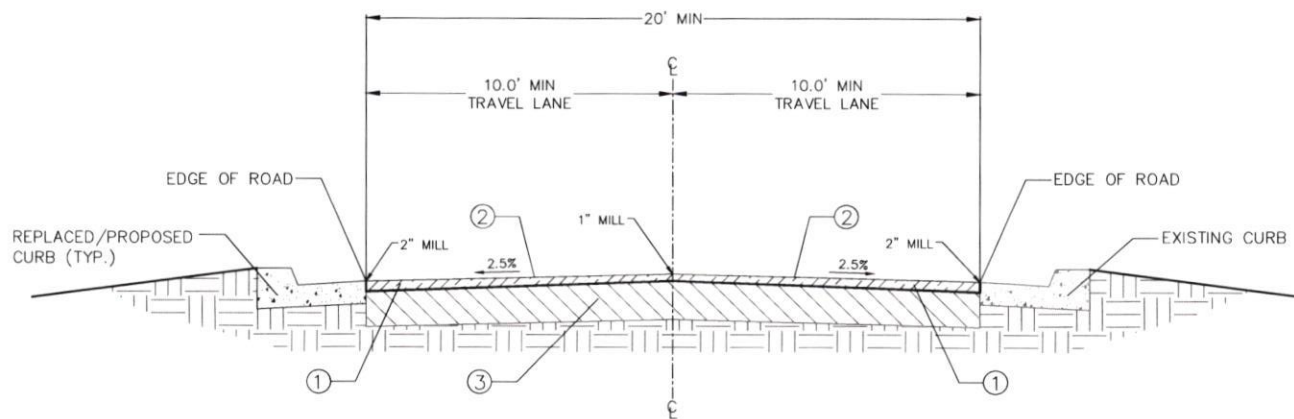
CHERRY LAUREL DR TYPICAL SECTION
