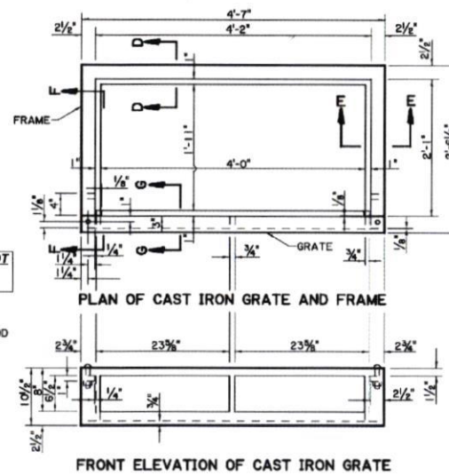
PLAN OF CAST IRON GRATE AND FRAME
