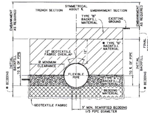
FLEXIBLE PIPE STORM DRAIN TRENCH AND EMBANKMENT INSTALLATIONS SCALE: 1\frac{1}{2}" = 1'-0"
