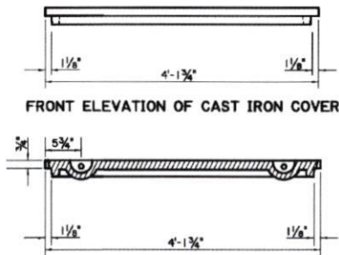
SECTION J-J
