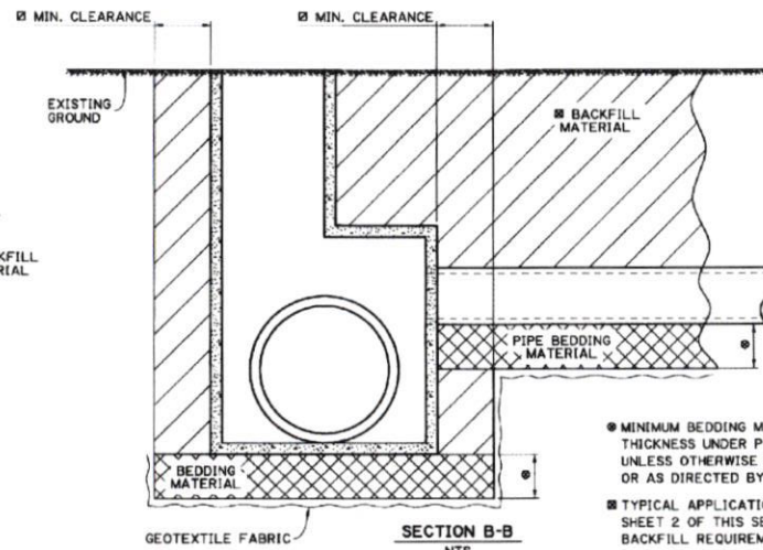
TYPICAL CATCH BASIN AND STORM SEWER PIPE INSTALLATION NTS
