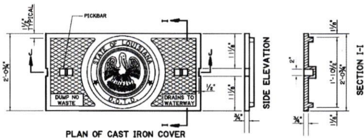
PLAN OF CAST IRON COVER
