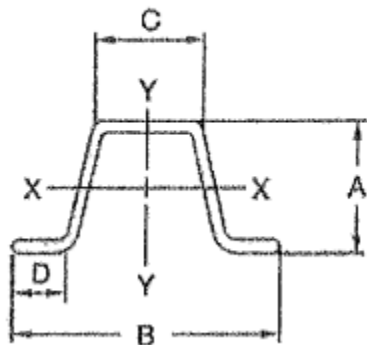
Sign Post and Base Post Weight - 2.50 lbs/ft
