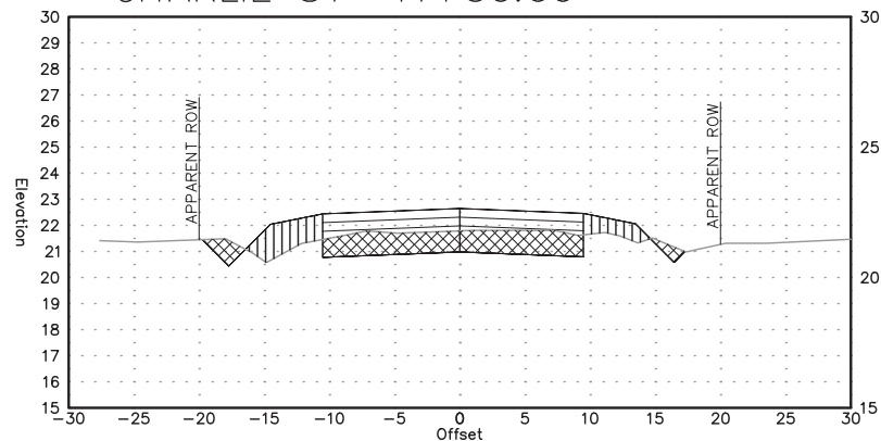
CHARLIE ST 11+50.00
