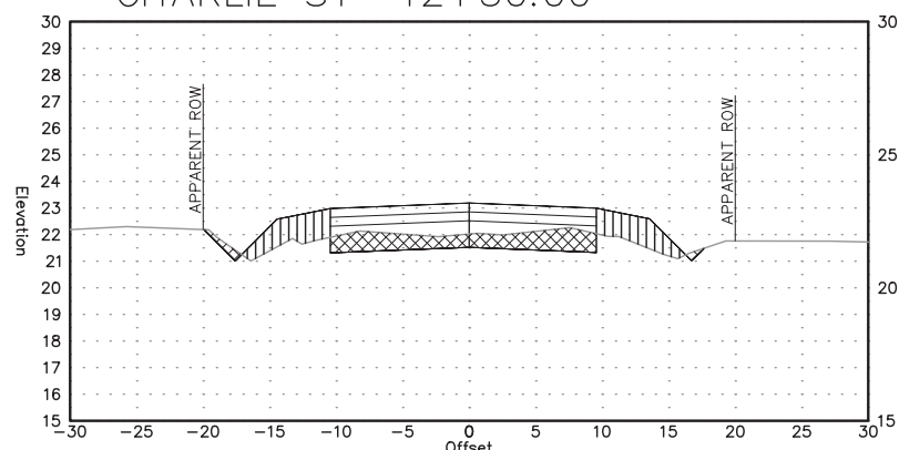
CHARLIE ST 12+50.00
