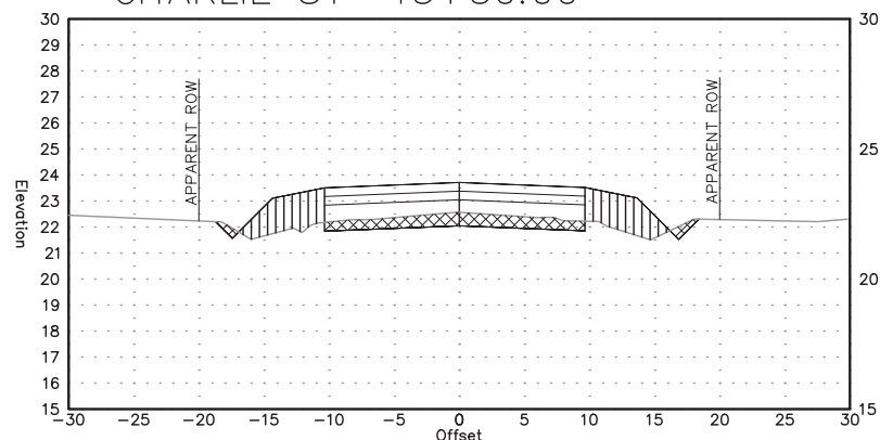
CHARLIE ST 13+50.00
