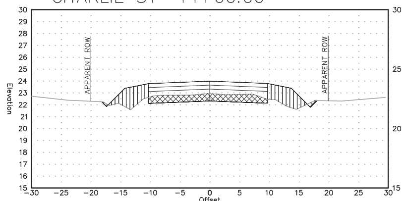
CHARLIE ST 14+00.00
