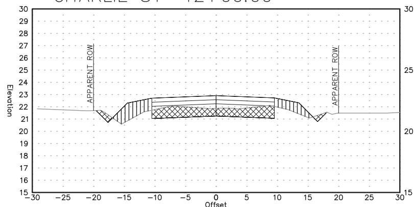
CHARLIE ST 12+00.00
