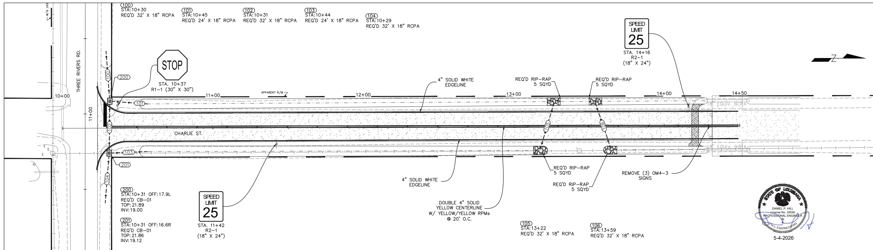
CHARLIE ST WEST PROFILE
