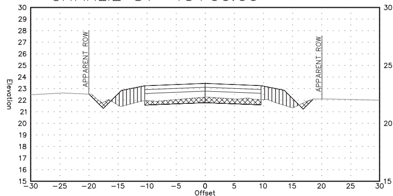
CHARLIE ST 13+00.00
