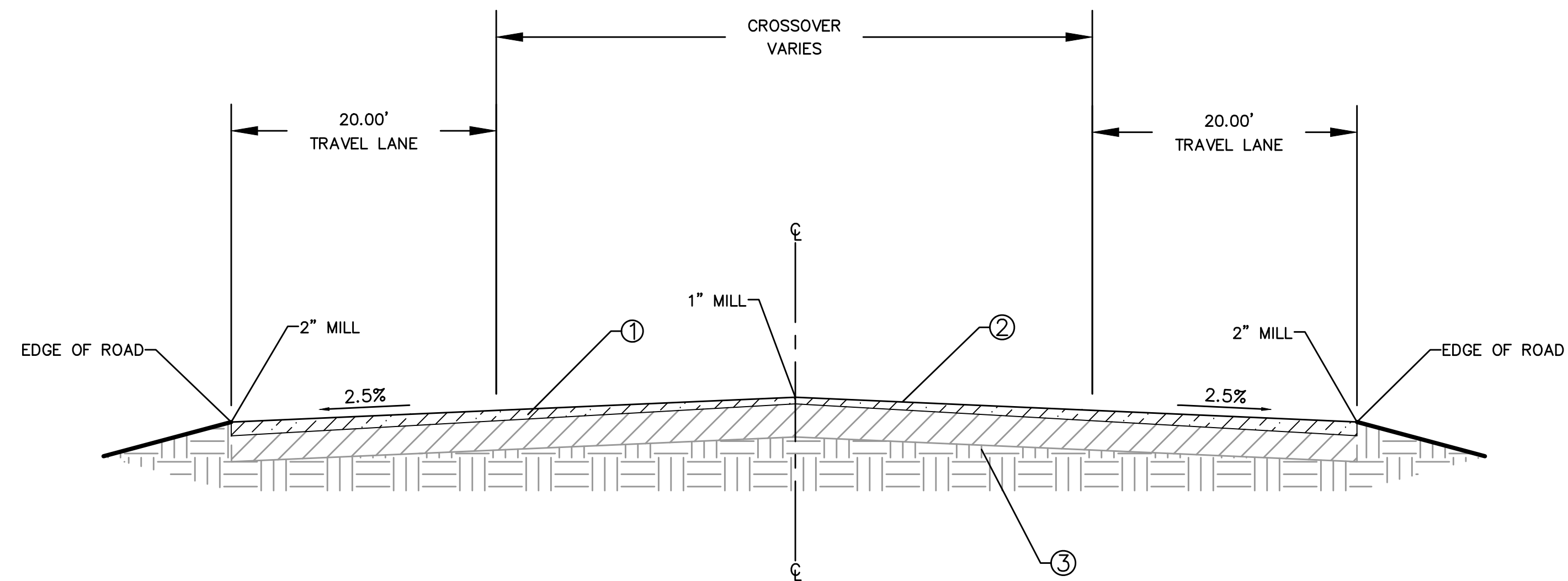
WOODRIDGE BLVD TYPICAL SECTION (CROSSOVER)
