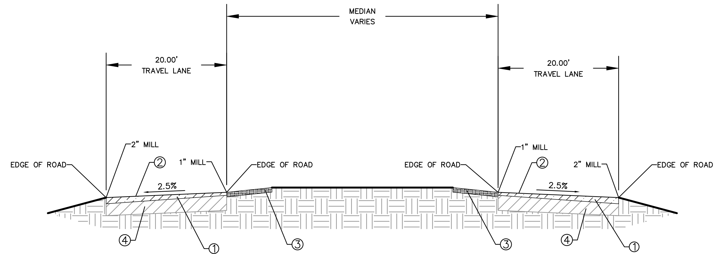
WOODRIDGE BLVD TYPICAL SECTION (BOULEVARD)
