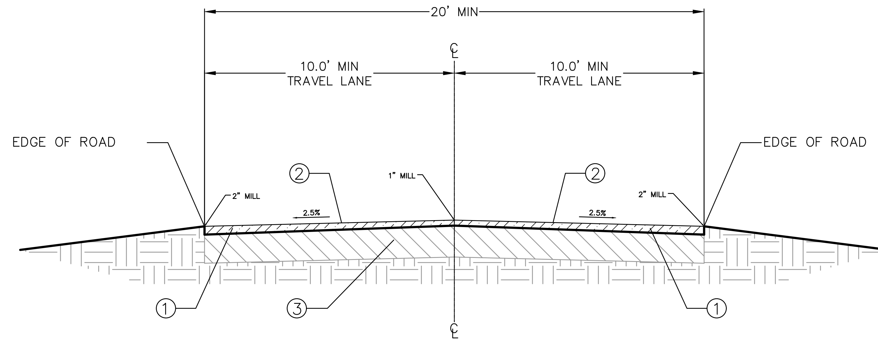
ENGLISH OAKS DR TYPICAL SECTION
