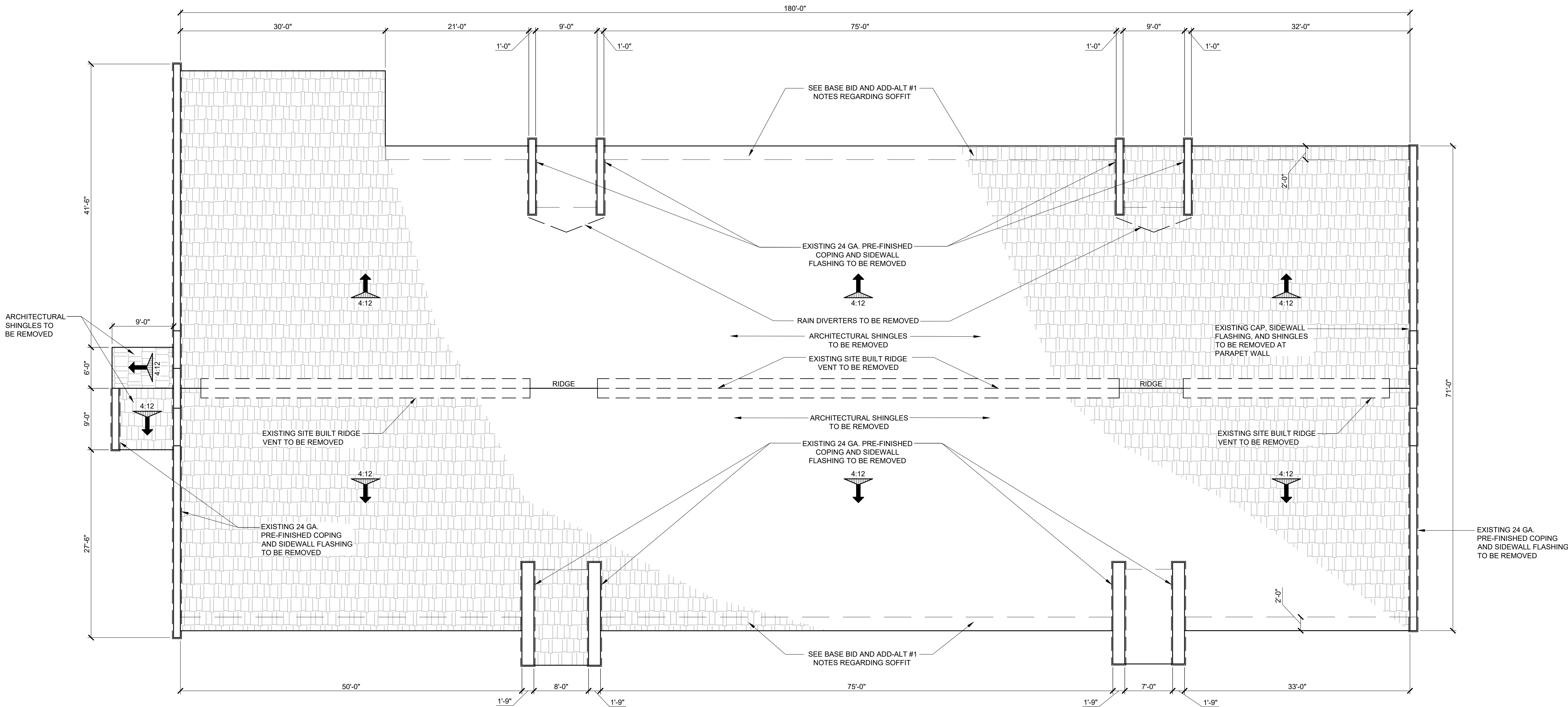
DEMOLITION ROOF PLAN SCALE: 1/8"=1'-0"
