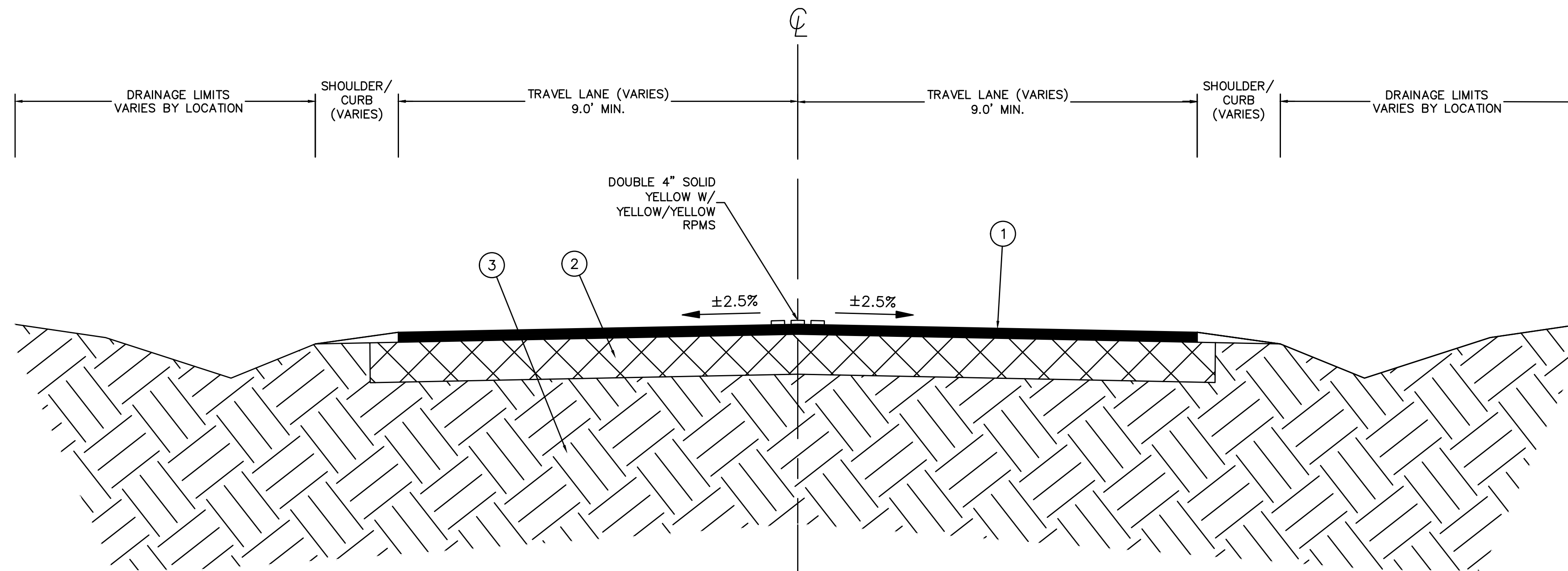
TYPICAL ROADWAY SECTION LOWE DAVIS RD STA 10+00 TO 117+57
