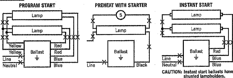
FIGURE A TYPICAL BALLAST CONFIGURATIONS
