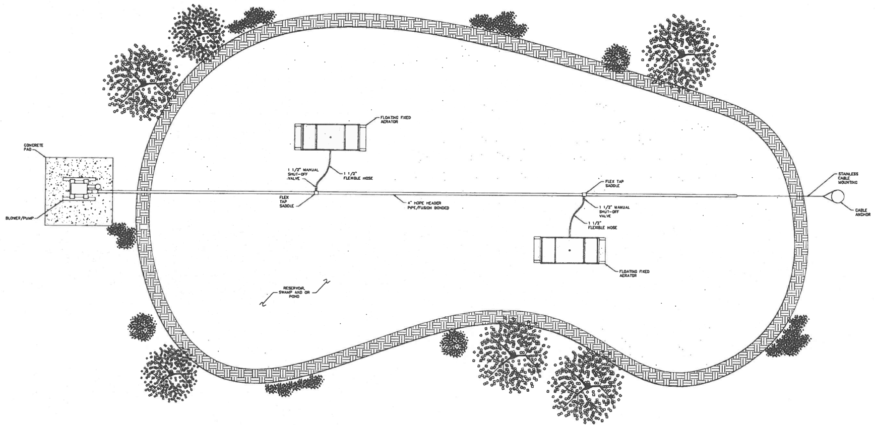
FIXED FILM AERATION UNIT INSTALLATION SCALE: NONE
