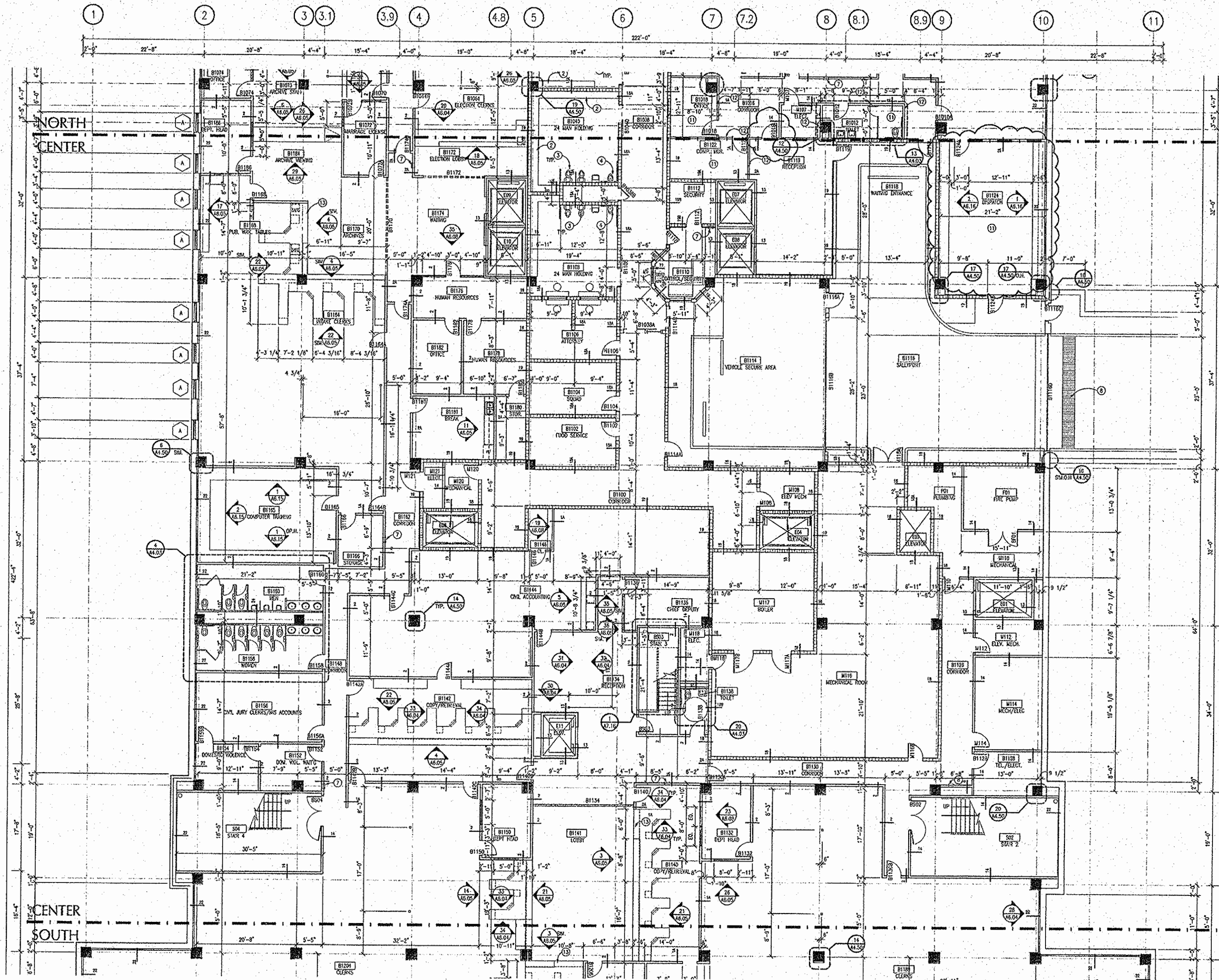
BASEMENT LEVEL CENTER - FLOOR PLAN
