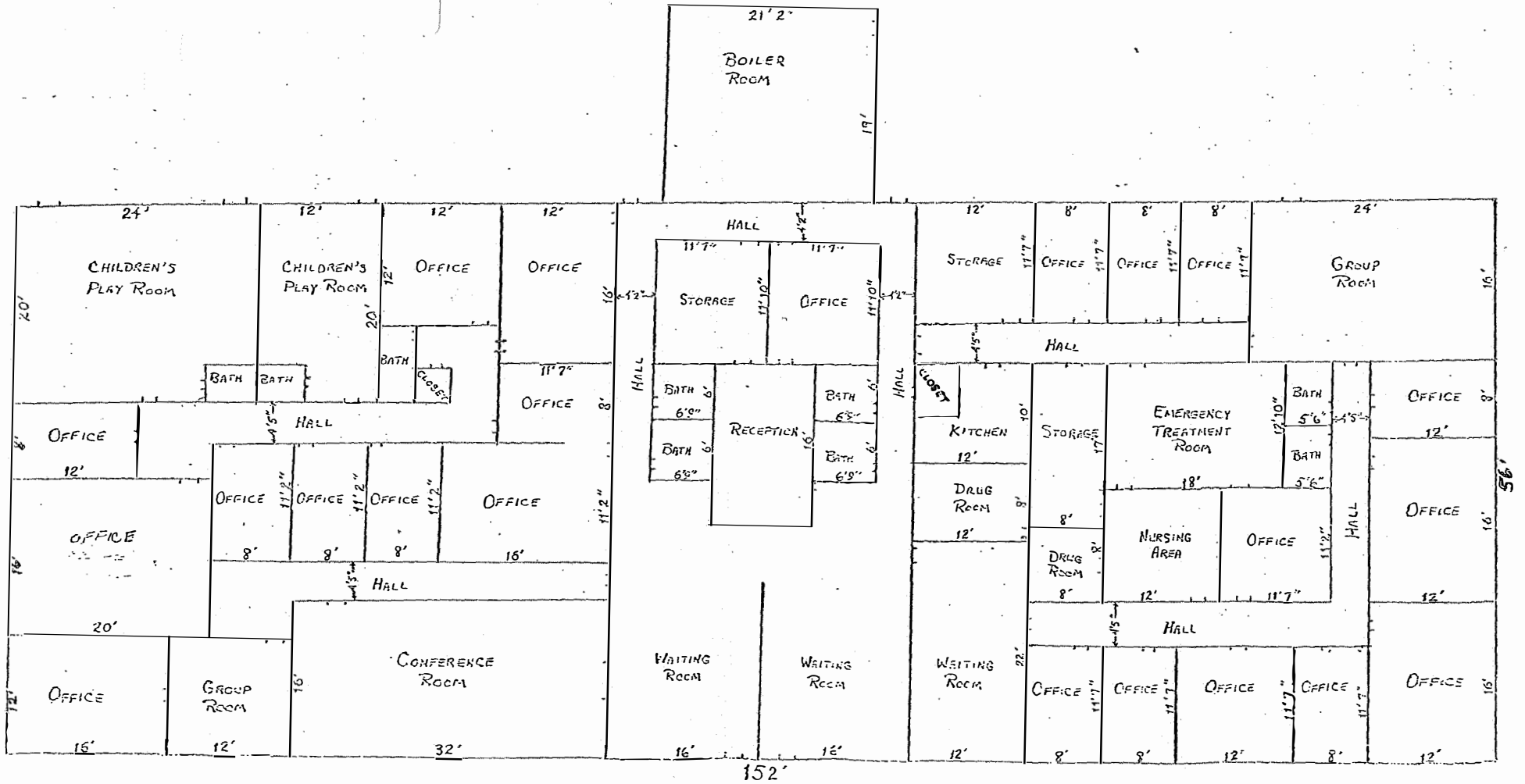
Floor Plan
