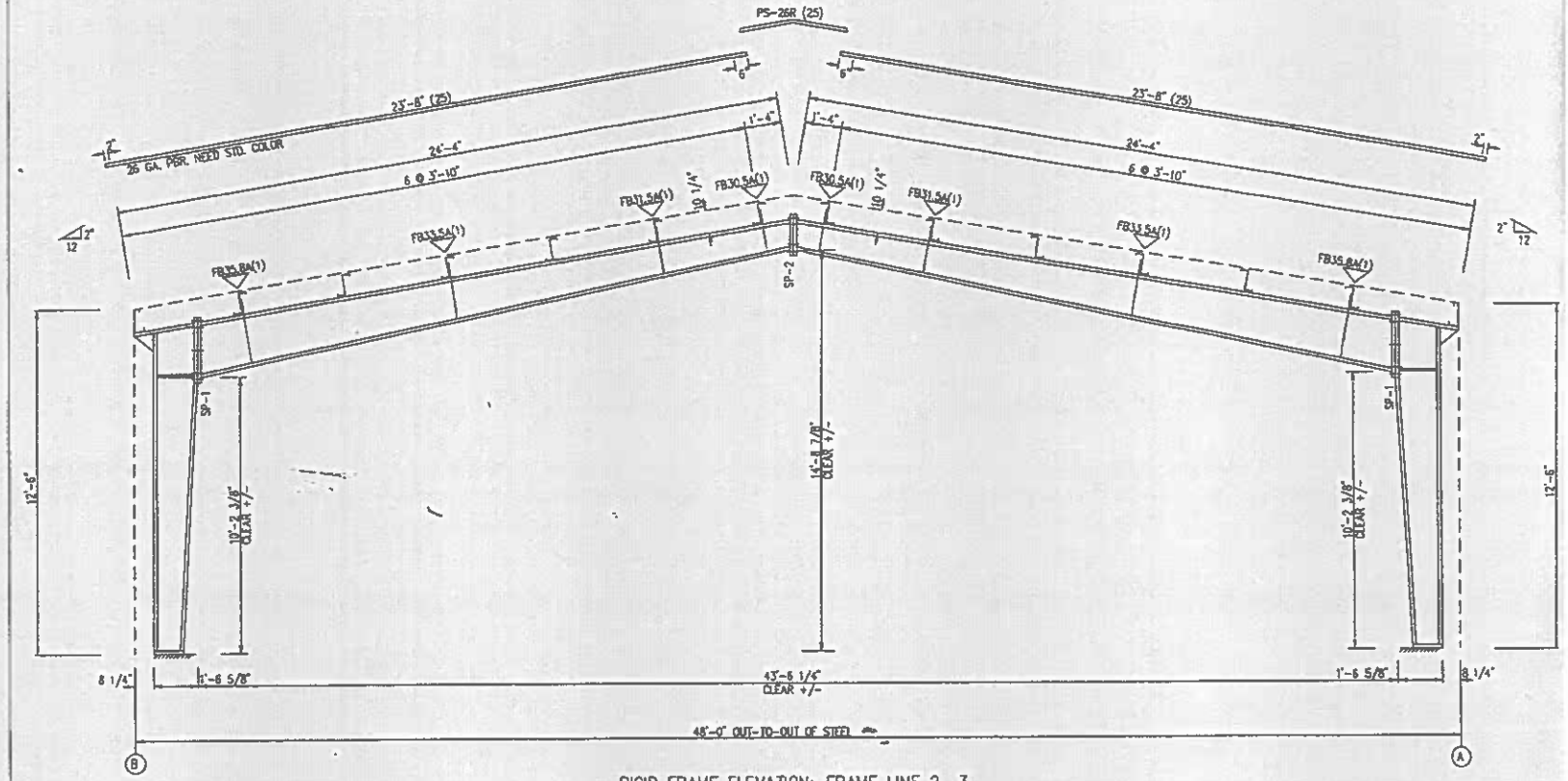
RIGID FRAME ELEVATION: FRAME LINE 2 3
