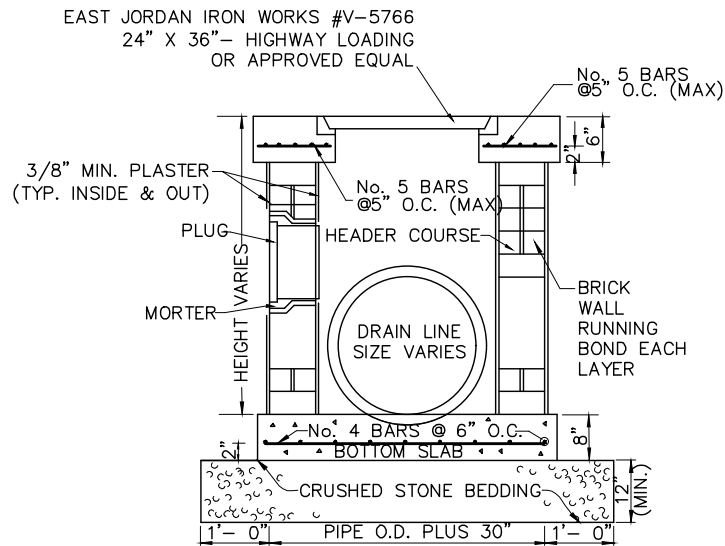
DRAIN INLET DETAIL
