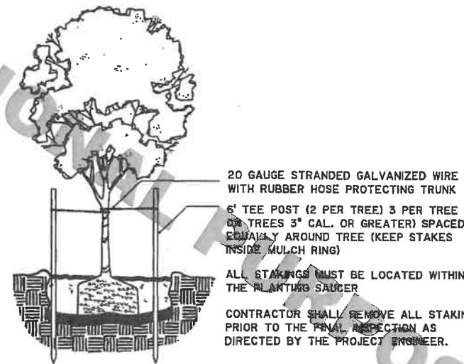
TREE STAKING DETAIL 4 NTS LD-1
