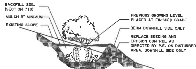
SLOPE PLANTING DETAIL 6 NTS LD-1
