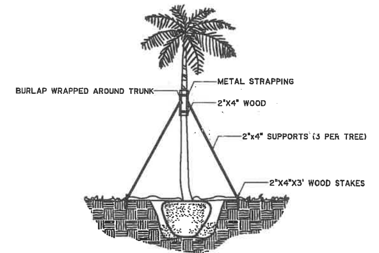
PALM STAKING DETAIL 5 NTS LD-1
